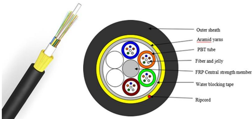
CABLE STRUCTURE AND PARAMETERS:
